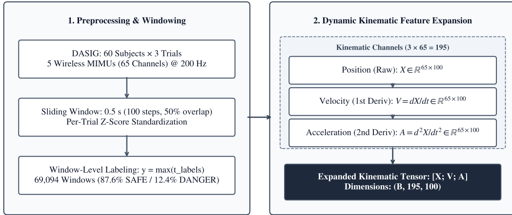
Fig. 2. Data preprocessing and dynamic feature expansion on the GPU.
